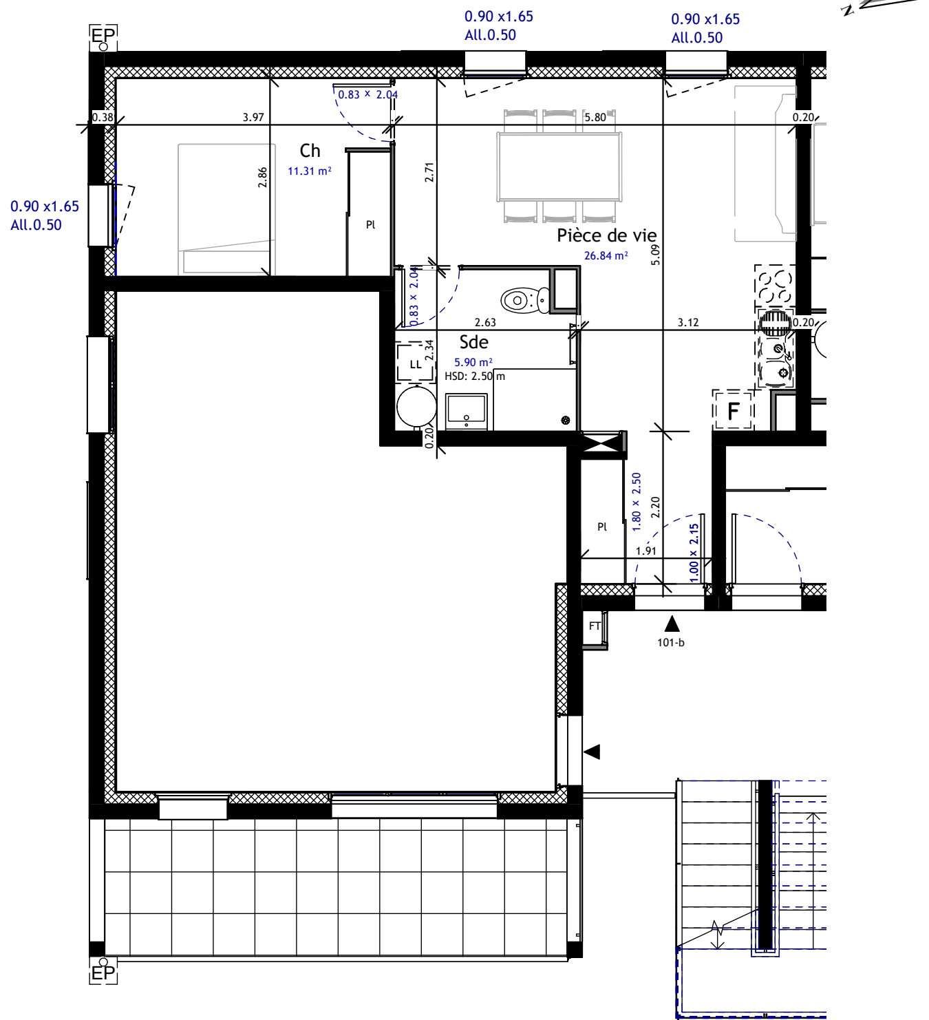
PLAN R+1 - A101-b
