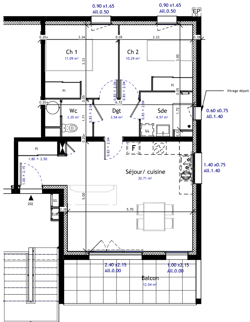
PLAN R+2 - C202
