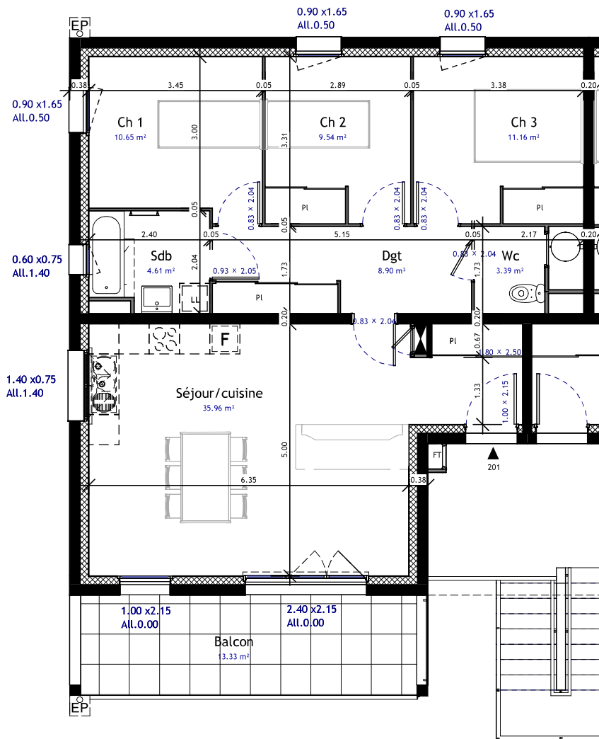
PLAN R+2 - C201
